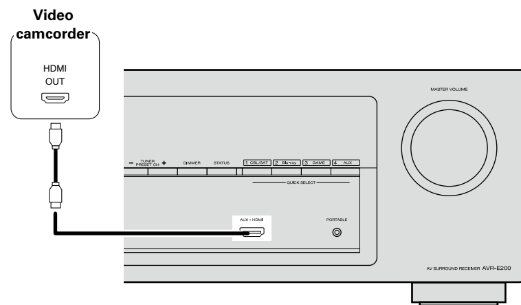
[Front panel]
